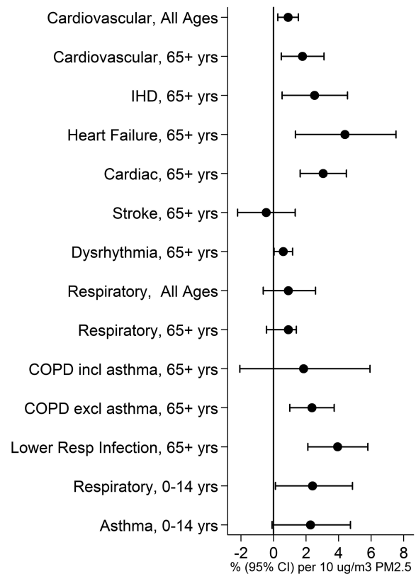
Figure 2 Summary estimates (95% confidence intervals) for cardiovascular and respiratory hospital admissions.
