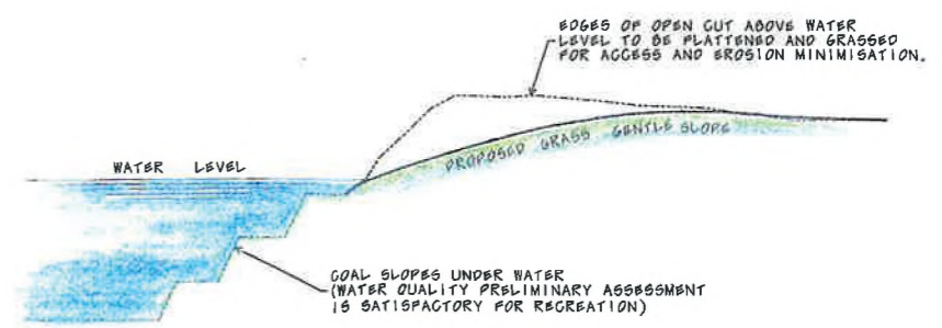
TYPICAL SECTION OF LAKE EDGE
